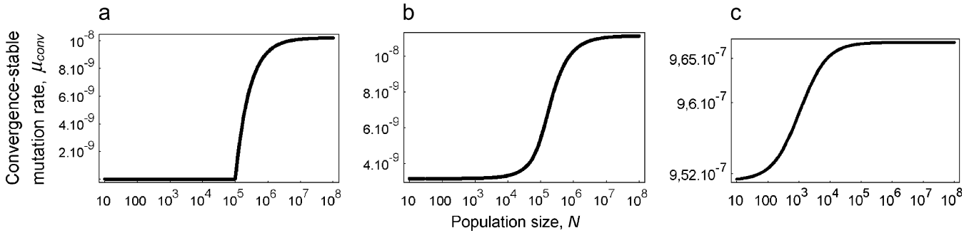
FIGURE 4.—Convergence stable mutation rate as a function of population size, in model B (Equation 26). The size of the deleterious genome is L = 10^5 ; the size of the adaptive genome is l = 10 ; the probability of fixation of adaptive mutations is \pi = 0.1 ; the rate of environmental changes is \epsilon = 10^{-3} ; and the cost of deleterious mutations is s_d = 0.05 . (a) The cost of accuracy is neglected ( f = 0 ); the population size has a threshold effect on convergence stable (CS) mutation rate. (b and c) The cost of accuracy is taken into account with f = 10^{-12} and 10^{-7} , respectively; the population size has a continuous and weak relative effect on CS mutation rate. Note that a, b, and c have different scales.
