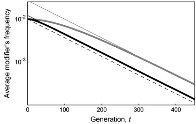
FIGURE 1.—The average modifier's frequency, plotted as a function of the number of generations after appearance, according to analytical models (thin lines) and to stochastic individual-based simulations (thick lines). The generation of deleterious mutations affects the modifier's frequency; the cost of accuracy and the existence of adaptive mutations are not considered. Simulations are performed with a population size N = 10^6 and are averaged over 10^4 runs. They are performed in two cases with different costs of deleterious mutations: s_d = 0.05 (thick solid line) and s_d = 0.01 (thick shaded line). The result of the analytical model neglecting the cost delay (Equation 14) is given by the dashed line. The results of the analytical model with delay (Equation 13) are given by the two thin lines, for each cost of deleterious mutation ( s_d = 0.05 and 0.01 , respectively, thin solid and thin shaded lines). Initial modifier's frequency is p(0) = 10^{-2} ; wild-type mutation rate is \mu = 10^{-6} ; modifier's effect is \delta = 10^{-6} ; and the deleterious genome has size L = 10^4 .
