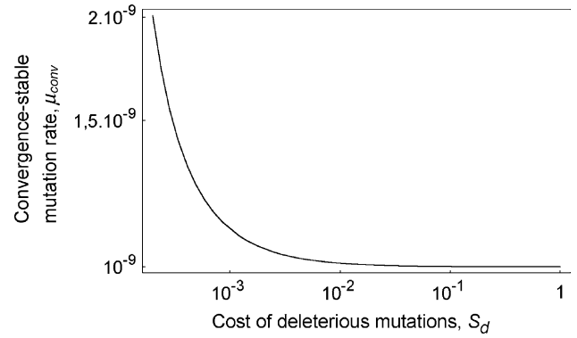
FIGURE 2.—Convergence stable mutation rate as a function of the fitness cost of each deleterious mutation in model A, under hypothesis 1 (advantageous mutations stronger than deleterious mutations, Equation 22). The size of the deleterious genome is L = 10^5 , the frequency of selective sweeps is K = 10^{-4} , and the cost of replication accuracy is absent ( f = 0 ).
