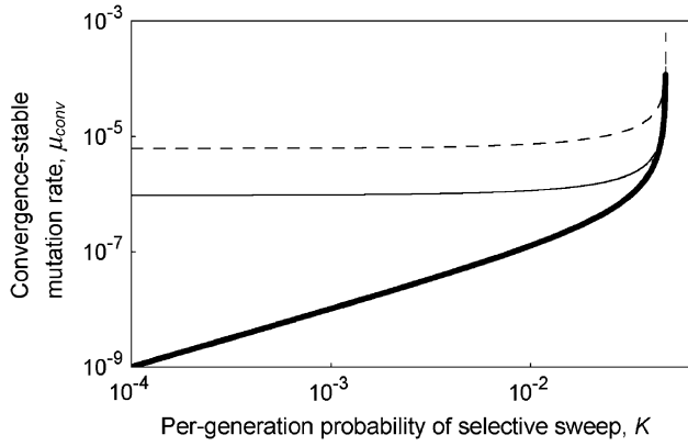
FIGURE 3.—Convergence stable mutation rate as a function of the rate of selective sweep in model A, under hypothesis 1 (advantageous mutations stronger than deleterious mutations, Equation 22). The size of the deleterious genome is L = 10^5 ; the cost of deleterious mutations is s_d = 0.05 . The cost of replication accuracy is characterized by f = 0 (no cost of accuracy, thick line), f = 10^{-7} (thin line), or f = 10^{-5} (dashed line).
